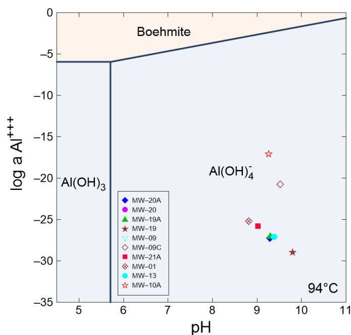
Figure 6: Stability diagram for aluminium species and boehmite at 94°C as a function of pH using The Geochemist's Workbench® (Bethke et al., 2024). Boehmite was generated after suppressing kaolinite, gibbsite, and diaspore.
